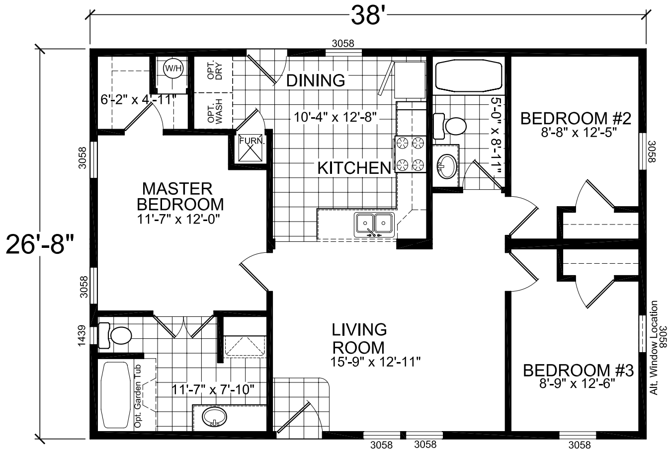
MODEL 418 3 BEDROOM, 2 BATH ACTUAL SIZE: 26'-8"x38'-0" TOTAL AREA: 1,013 SQ. FT.
